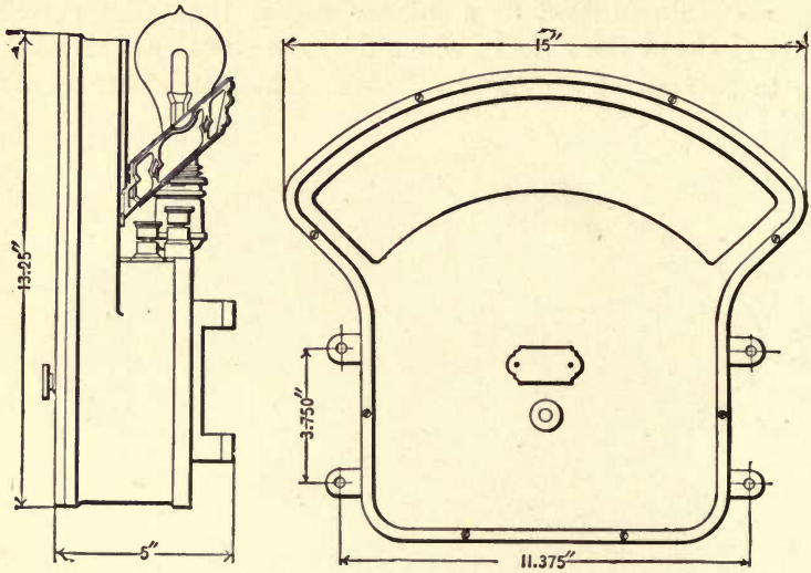
Fig. 92.—Illuminated-Dial Voltmeter
